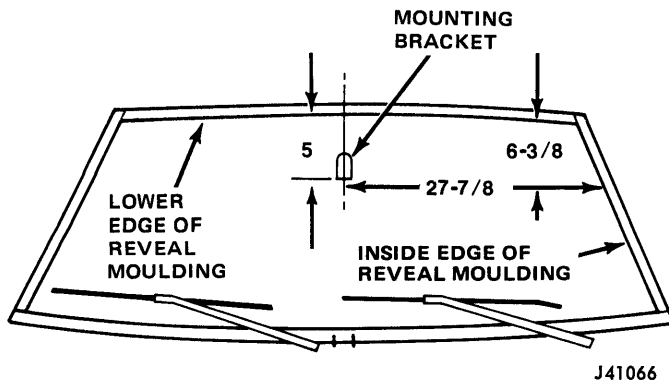
Fig. 17-6 Windshield Mounted Rear View Mirror Bracket Location (Inches)—Cherokee-Wagoneer-Truck
