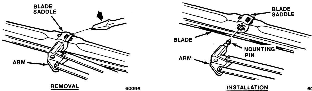
Fig. 17-9 Wiper Blade Replacement
