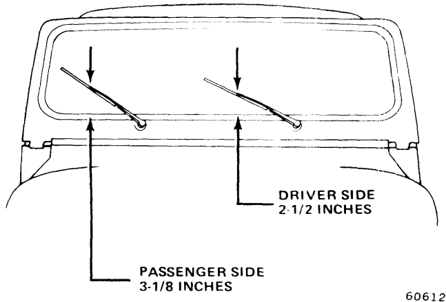
Fig. 17-11 Wiper Arm Park Position—CJ Models
